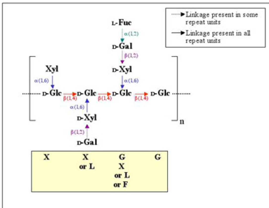
Figure 2. Acceptor structure of XG backbone decorated with galactosyl and fucosyl residues. This structure of XG is typical of that found in many dicots. This representation simplifies XG structure and is not intended to convey all the topological nuances.
