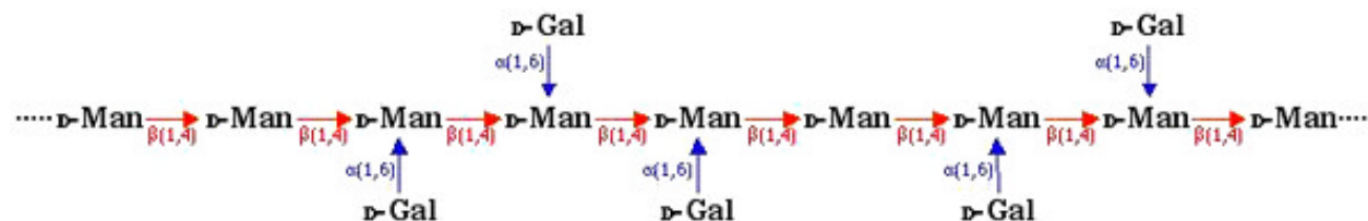
Figure 3. An overview of the branching pattern of the less abundant noncellulosic polysaccharide galactomannans; a backbone composed exclusively of (1,4) \beta -D-mannose decorated with \alpha -D-galactosyl units added at the O-6 positions.
